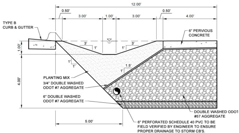
BIOSWALE CELL SECTION (TYP.)
