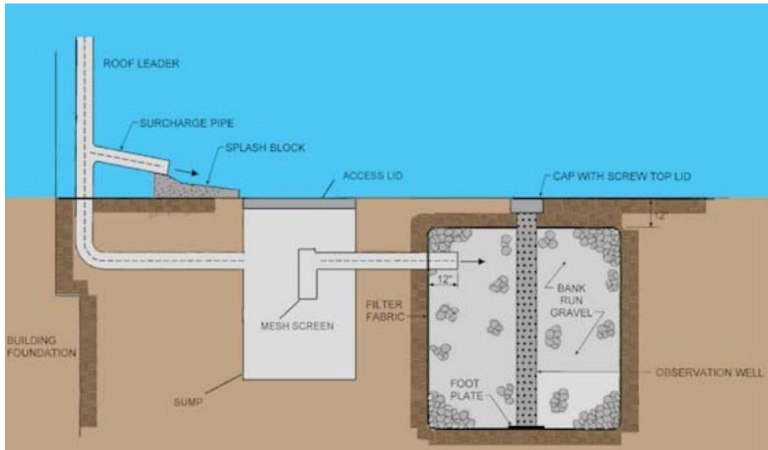
Figure 12. Dry Well or Seepage Pit
