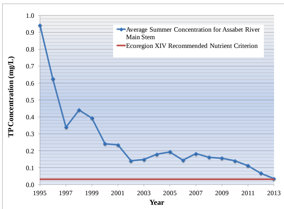
Figure 2. Average Summer TP Concentrations for the Main Stem of the Assabet River (OARS data)
